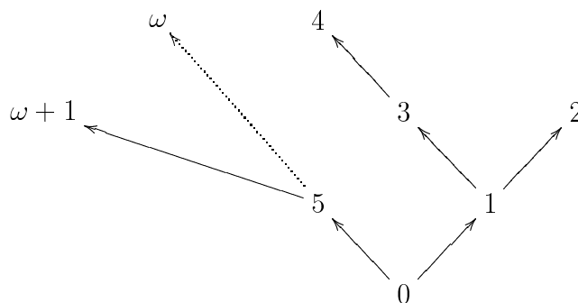
FIGURE 1. An almost linear iteration tree
