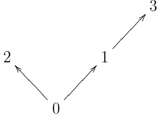
FIGURE 2. A normal tree generated by 0^\dagger
