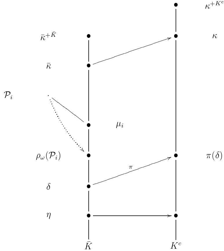
FIGURE 3. The covering argument
